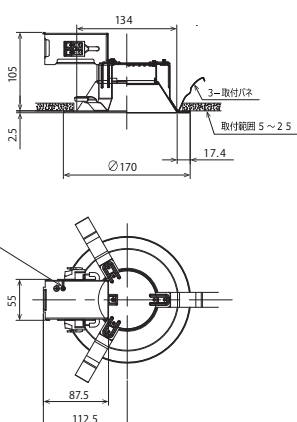
LRS1-05 Reach-D-100-6A Reach-D-100-6A D 調光可能型 (PWM)
